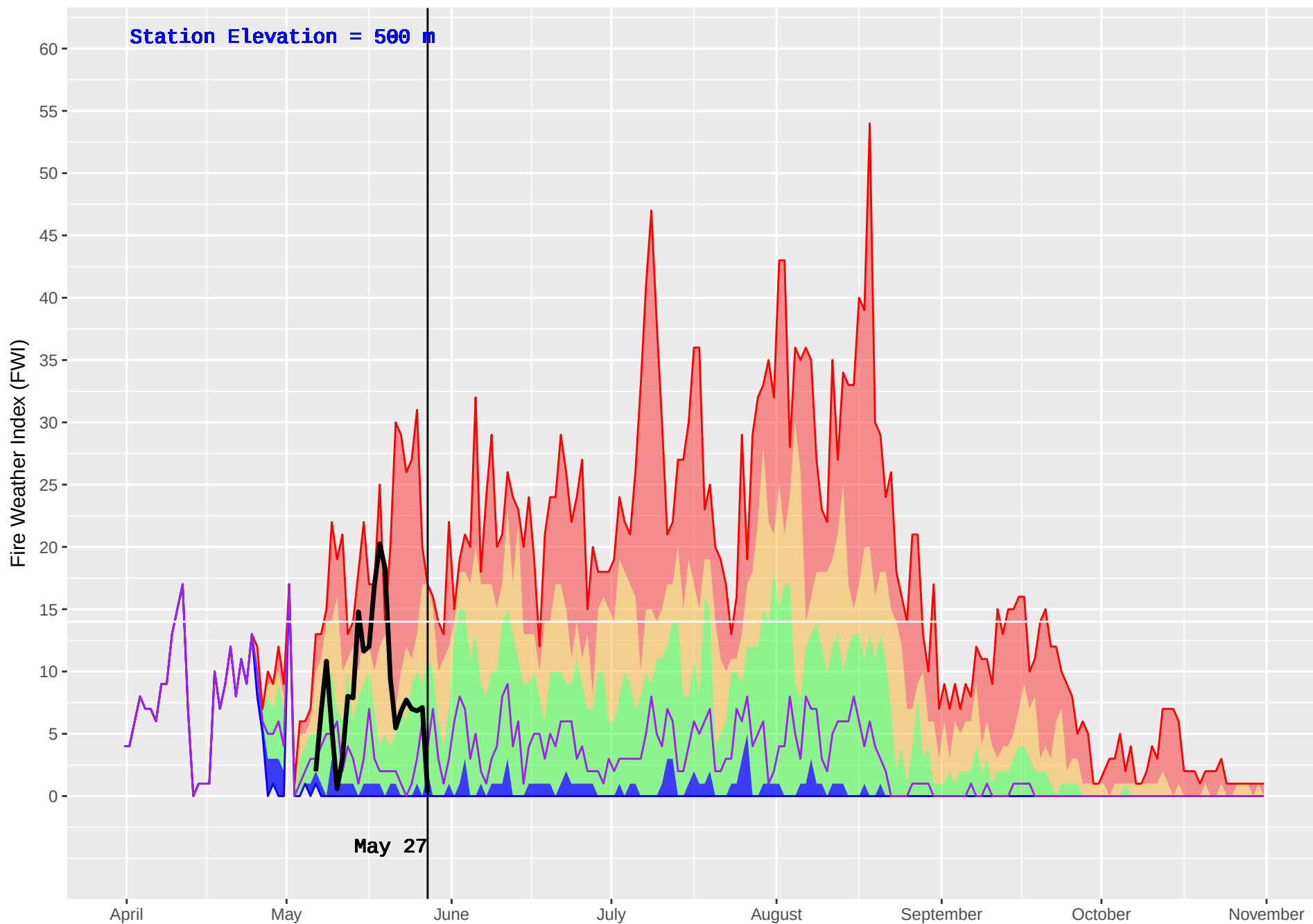
CRANBERRY (433) : Historical (1995–2016) and Current (2018) Noon Fire Weather Index (FWI)
