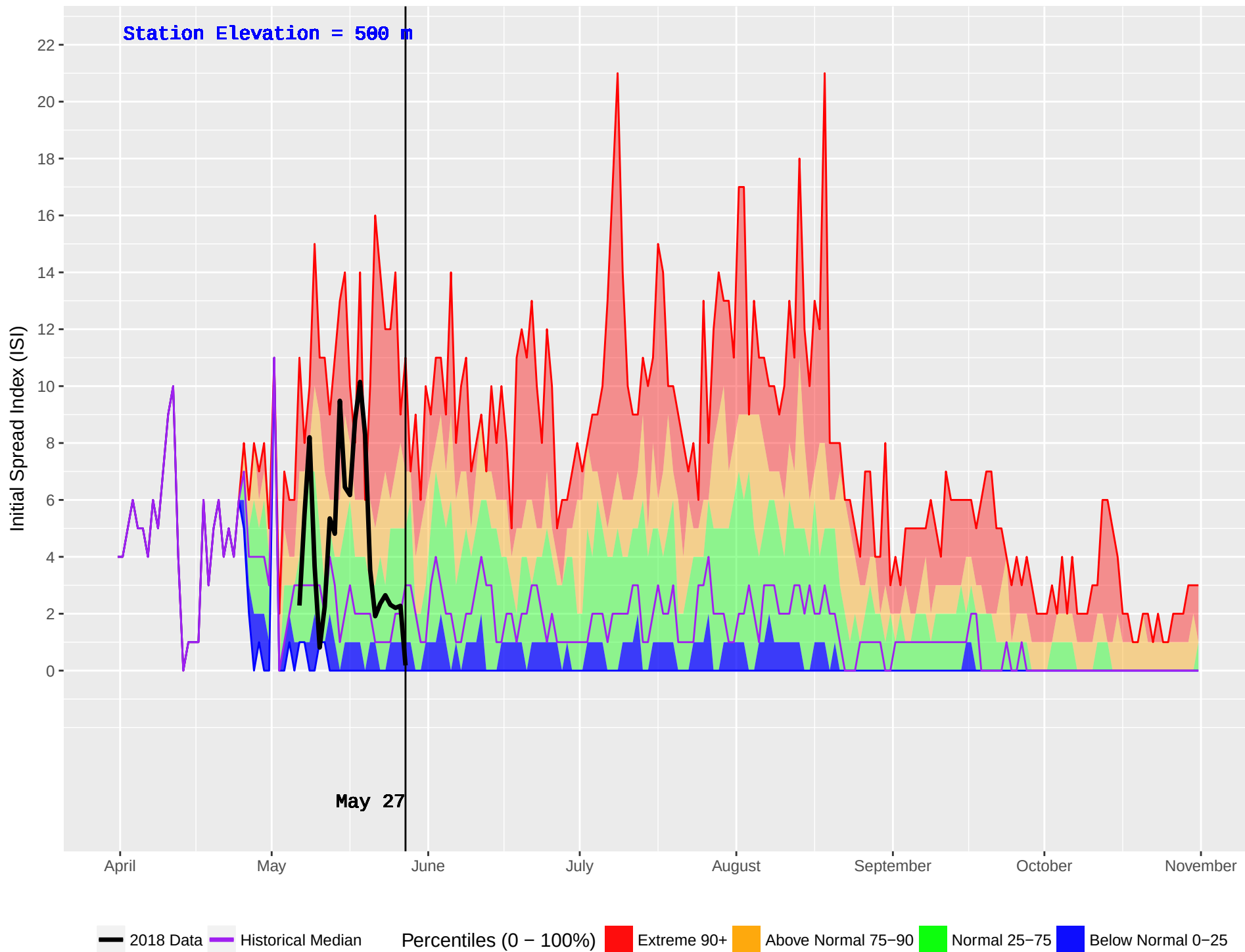
CRANBERRY (433) : Historical (1995–2016) and Current (2018) Noon Initial Spread Index (ISI)
