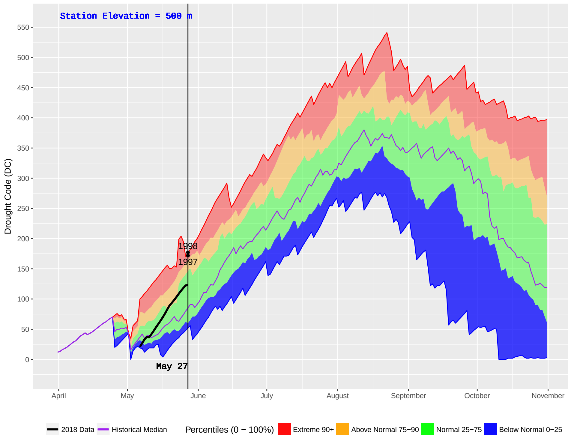
CRANBERRY (433) : Historical (1995–2016) and Current (2018) Noon Drought Code (DC)
