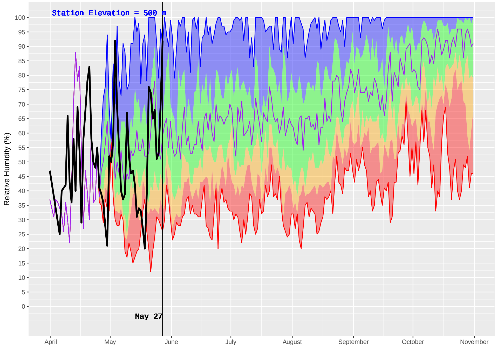
CRANBERRY (433) : Historical (1995–2016) and Current (2018) Noon Relative Humidity
