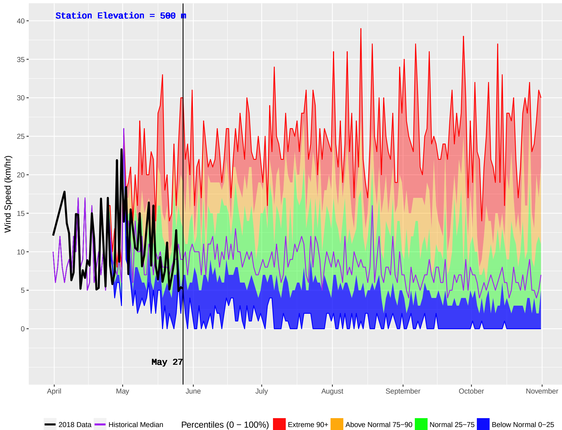
CRANBERRY (433) : Historical (1995–2016) and Current (2018) Noon Wind Speed
