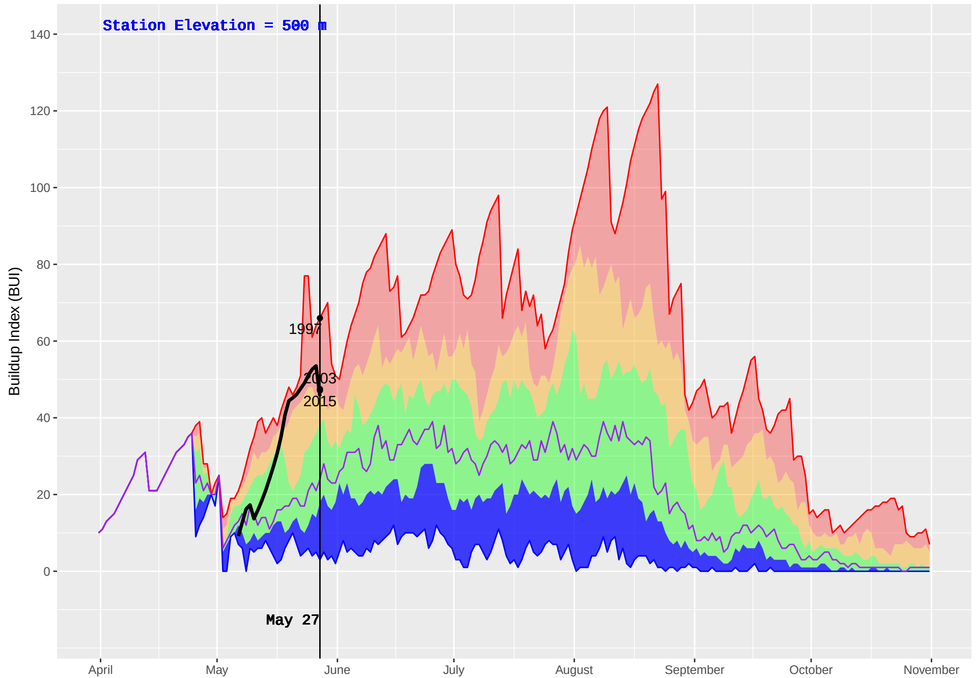
CRANBERRY (433) : Historical (1995–2016) and Current (2018) Noon Buildup Index (BUI)
