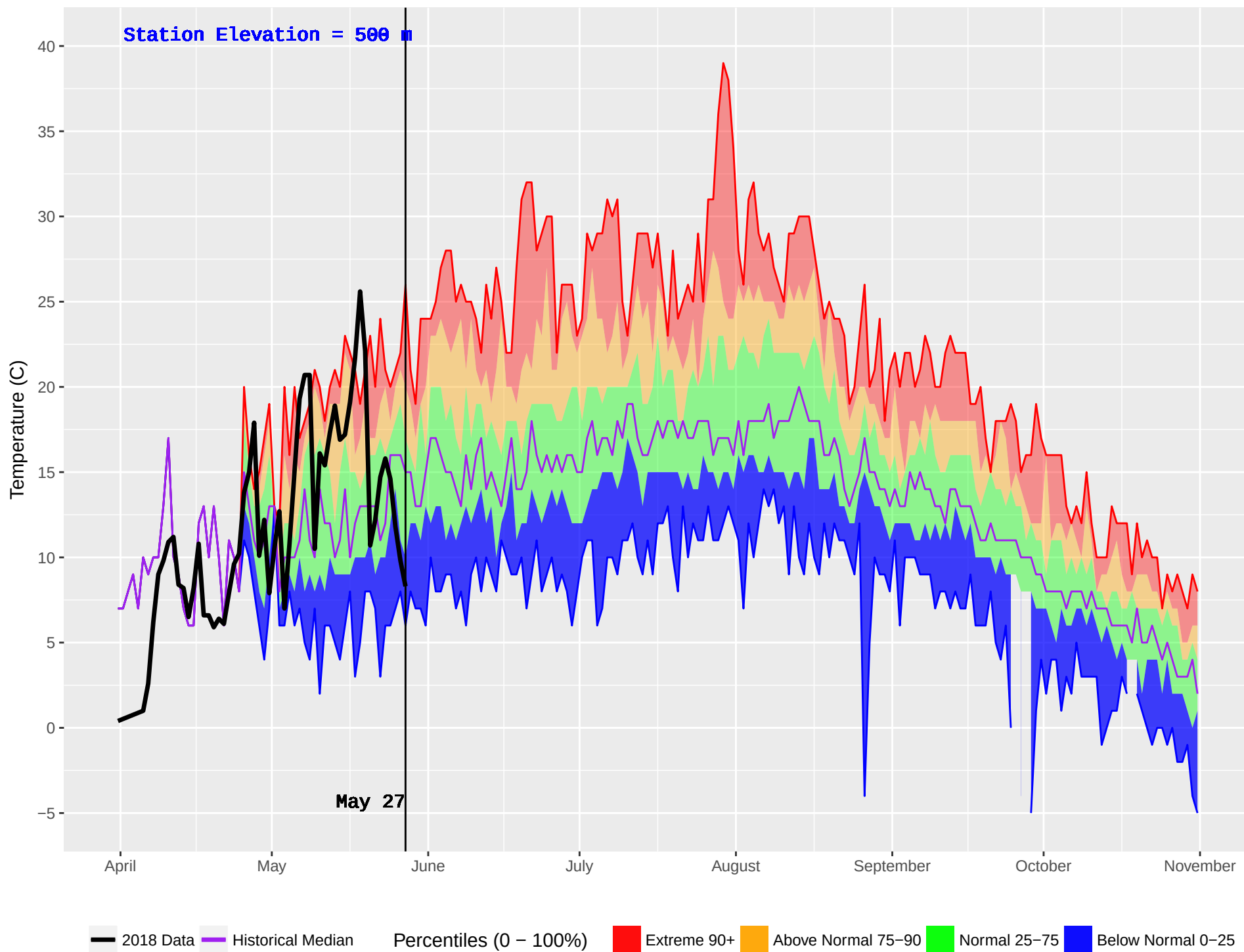
CRANBERRY (433) : Historical (1995–2016) and Current (2018) Noon Temperature
