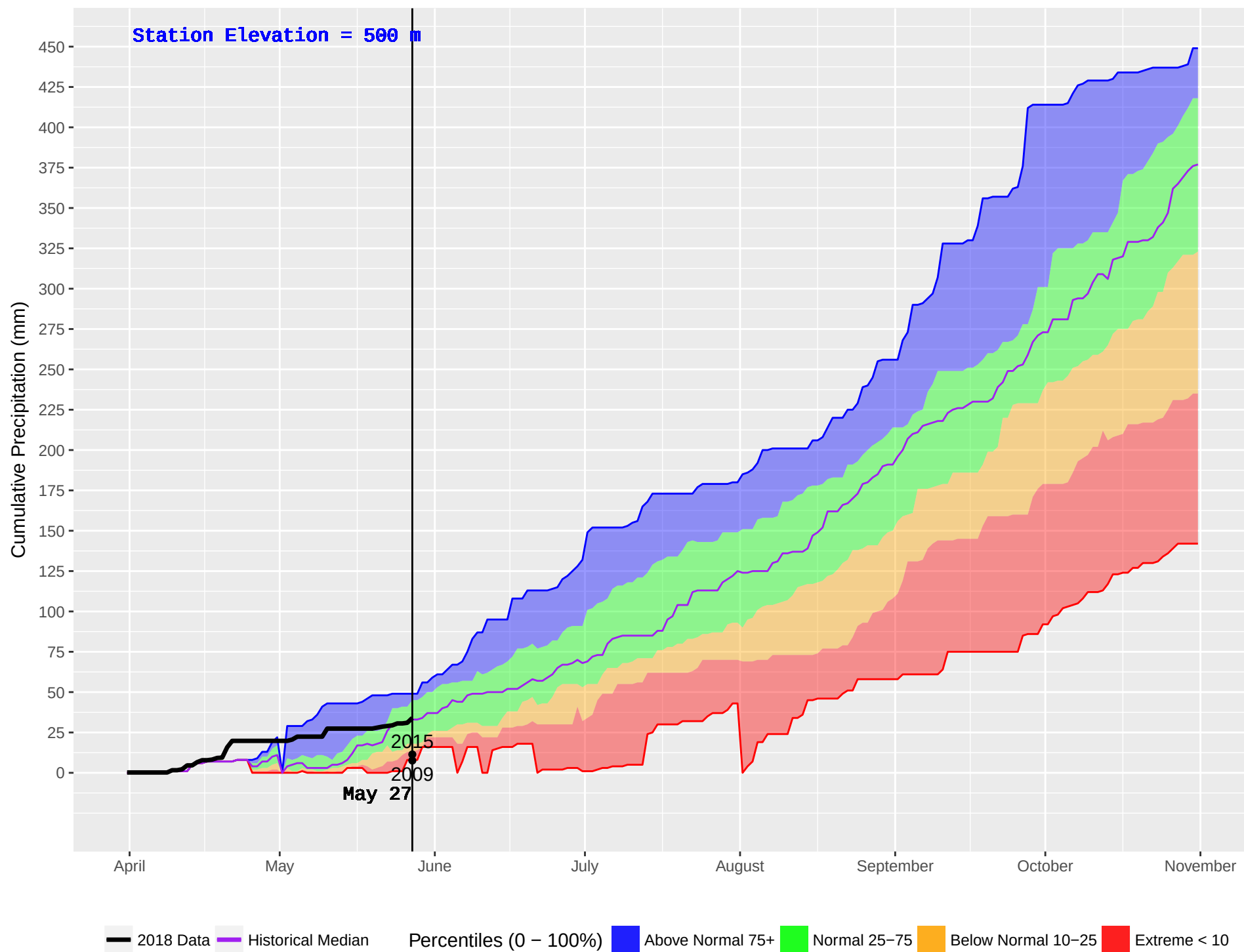
CRANBERRY (433) : Historical (1995–2016) and Current (2018) Noon Cumulative Precipitation
